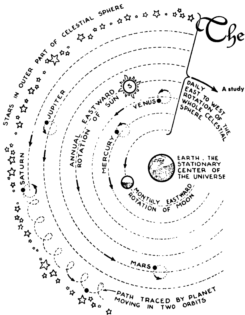
Fig. 1. Ptolemy's picture of the structure and relative motions of the members of the universe.
